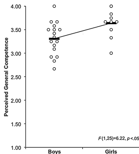
Fig. 2. Gender as a predictor of perceived general competence.
