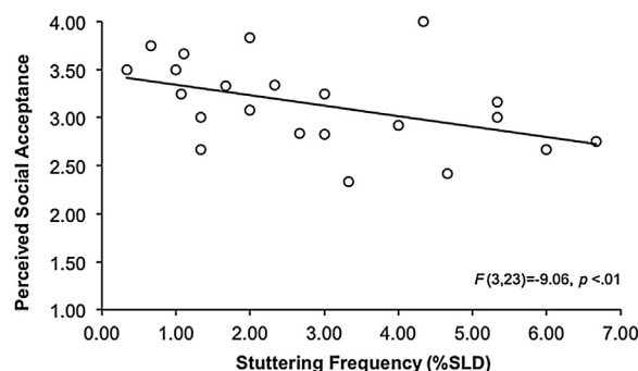
Fig. 3. Stuttering frequency as a predictor of perceived social acceptance.
