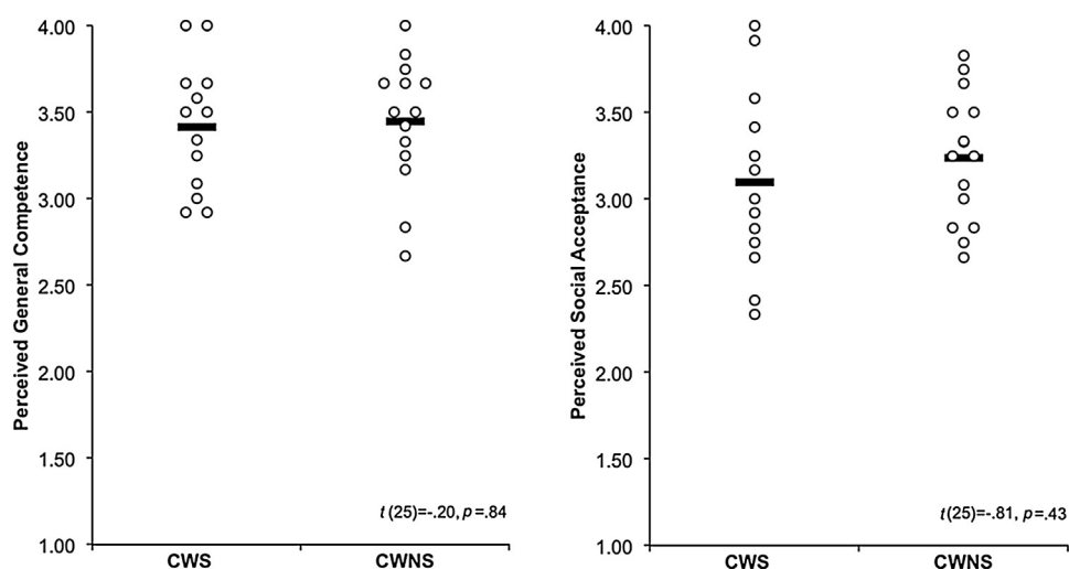
Fig. 1. PSPCSA composite scores by group.
